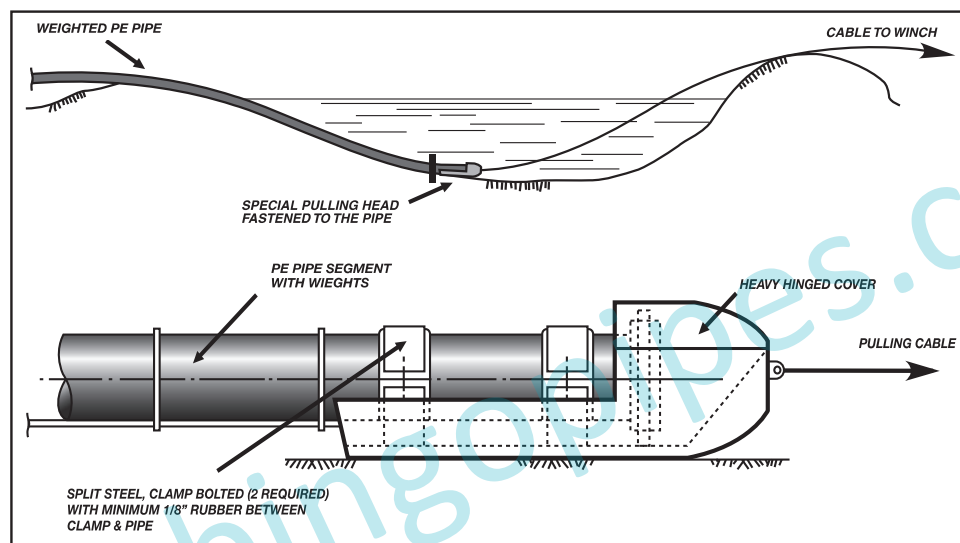
Figure 6 “Bottom-Pull” Installation of PE Pipe
