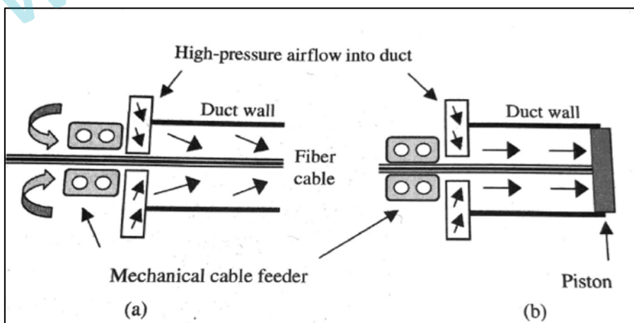
Figure 15 On left, Push-Blow (aka Jetting) Method. On right, Push-Pull Method
