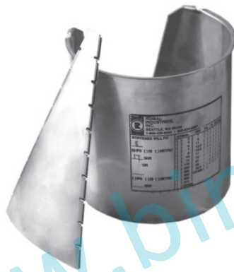
Figure 18 Split Ring Stiffener for PE pipe
