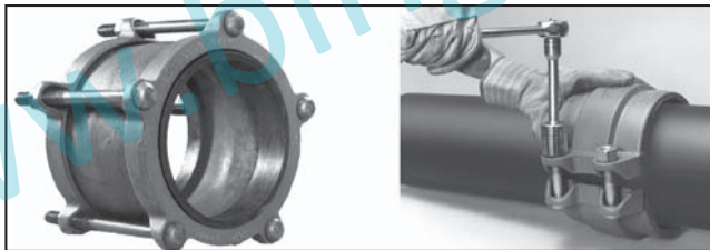
Figure 6 Mechanical Couplings
